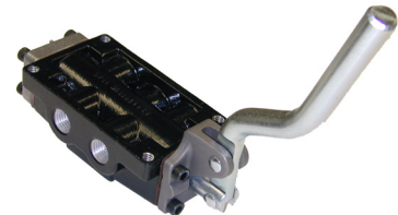
638VY - ref# 8185581 Bead Loosener (Spring Center)
